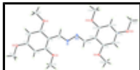
Fig. 1. The molecular structure of the title compound, showing 50% probability displacement ellipsoids and the atom-numbering scheme. Atoms with suffix A were generated by symmetry code -x, 2 - y, 1 - z .
